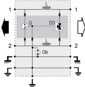
P: 3-electrode gas tube PB: 2-electrode gas tube L: Inductor D: Clamping diode
